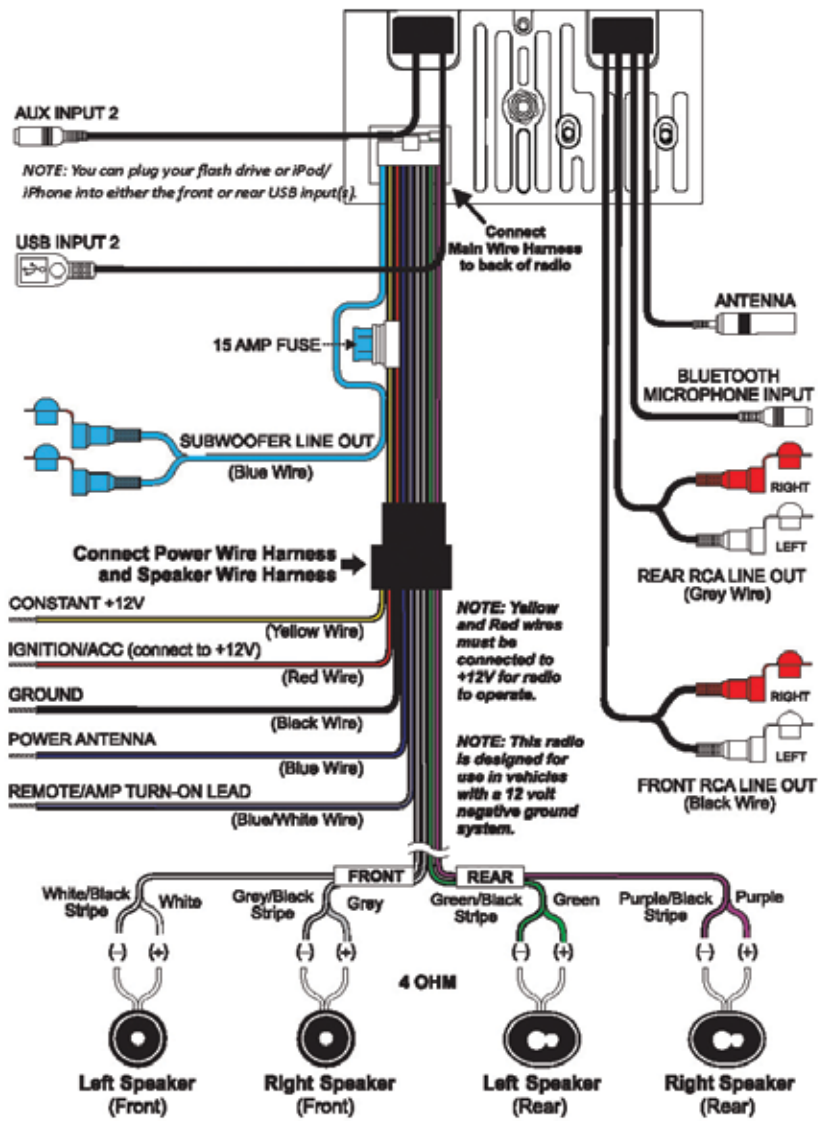
Figure 2 - Wiring Diagram
