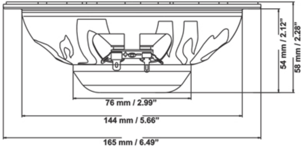
6.5" midbass drivers w/ wire mesh grilles
